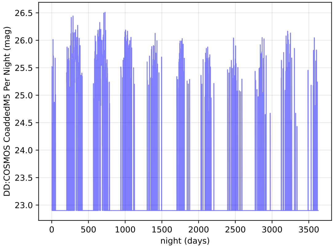
ddf_acor_sf15_lsf40_lsr20_v3.4_10yrs r band: DD:COSMOS CoaddedM5 Per Night
