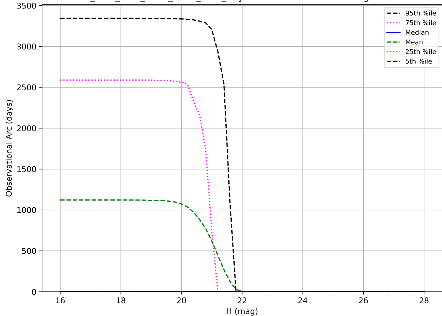
ddf_acor_sf15_lsf40_lsr10_v3.4_10yrs: Observational Arc Length Vatira
