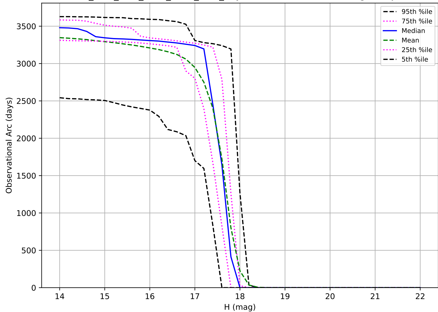
ddf_acor_sf15_lsf40_lsr10_v3.4_10yrs: Observational Arc Length Trojan
