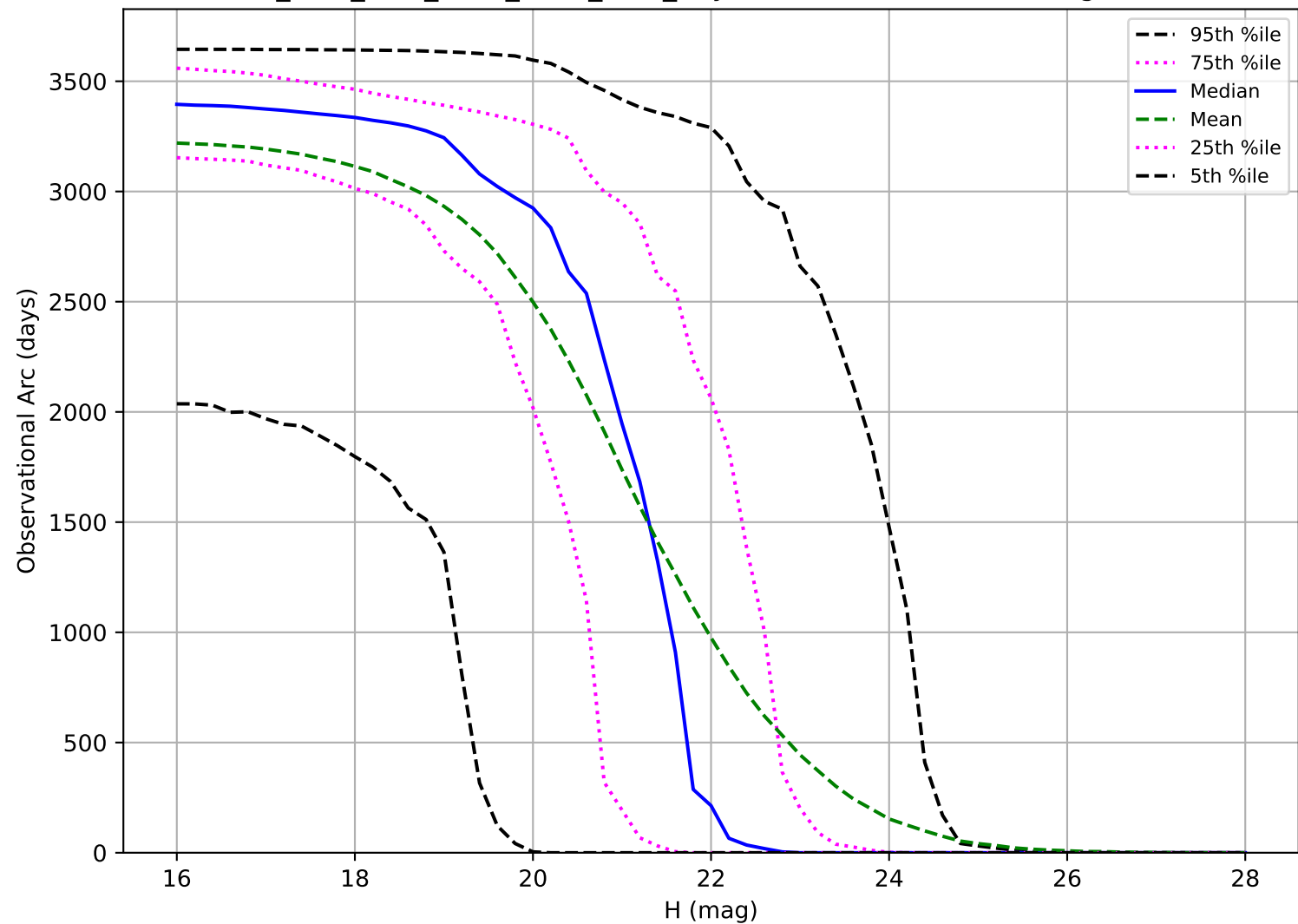
ddf_acor_sf15_lsf40_lsr10_v3.4_10yrs: Observational Arc Length PHA
