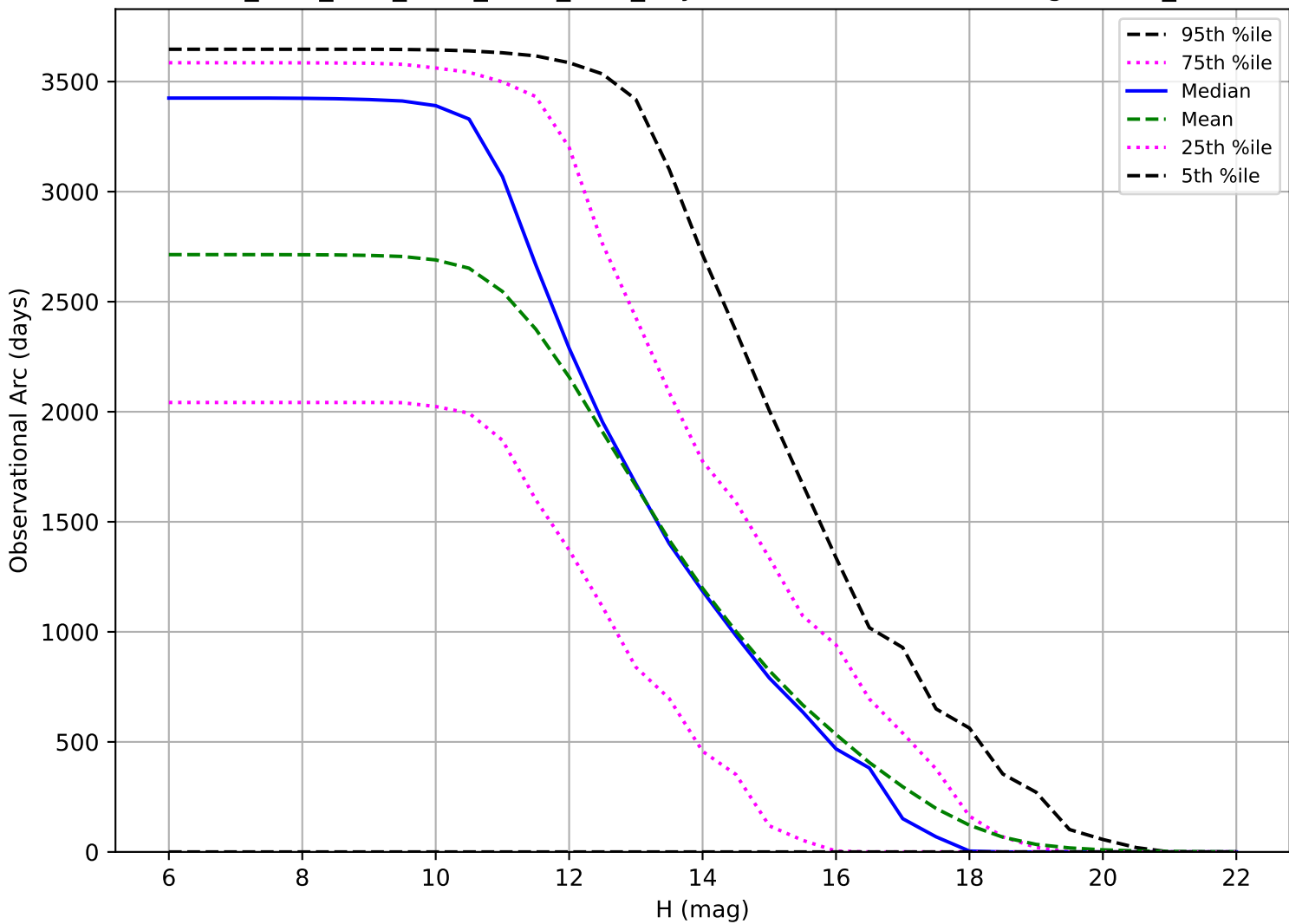
ddf_acor_sf15_lsf40_lsr10_v3.4_10yrs: Observational Arc Length OCC_r5
