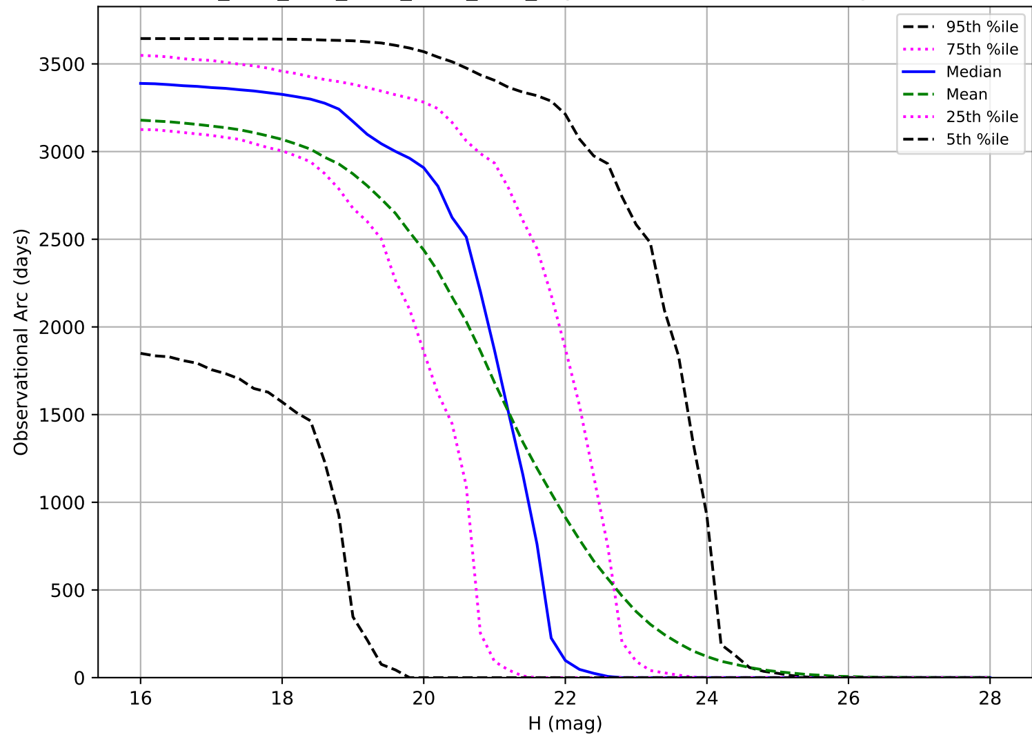
ddf_acor_sf15_lsf40_lsr10_v3.4_10yrs: Observational Arc Length NEO
