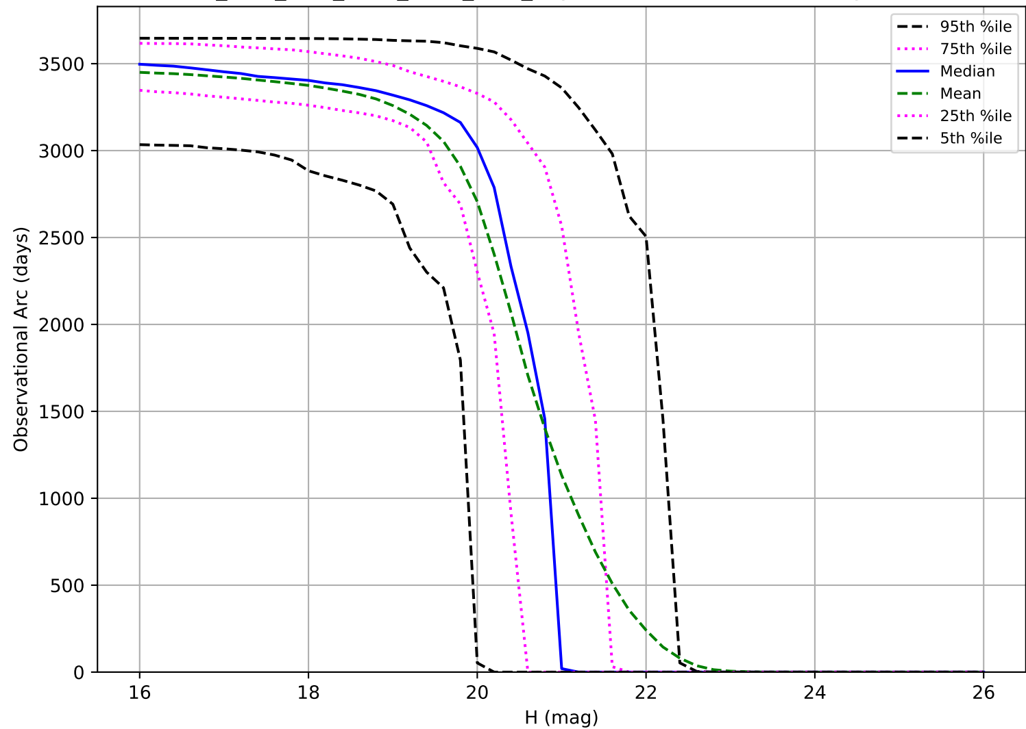
ddf_acor_sf15_lsf40_lsr10_v3.4_10yrs: Observational Arc Length MBA
