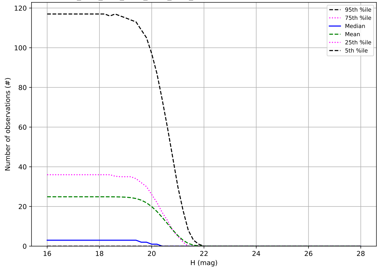
ddf_acor_sf15_lsf40_lsr10_v3.4_10yrs: Number of observations Vatira
