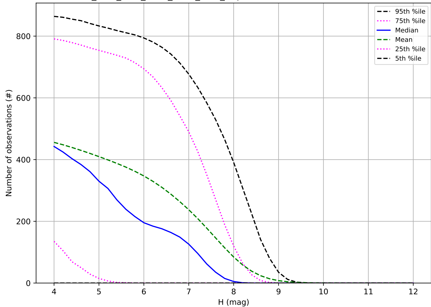
ddf_acor_sf15_lsf40_lsr10_v3.4_10yrs: Number of observations TNO
