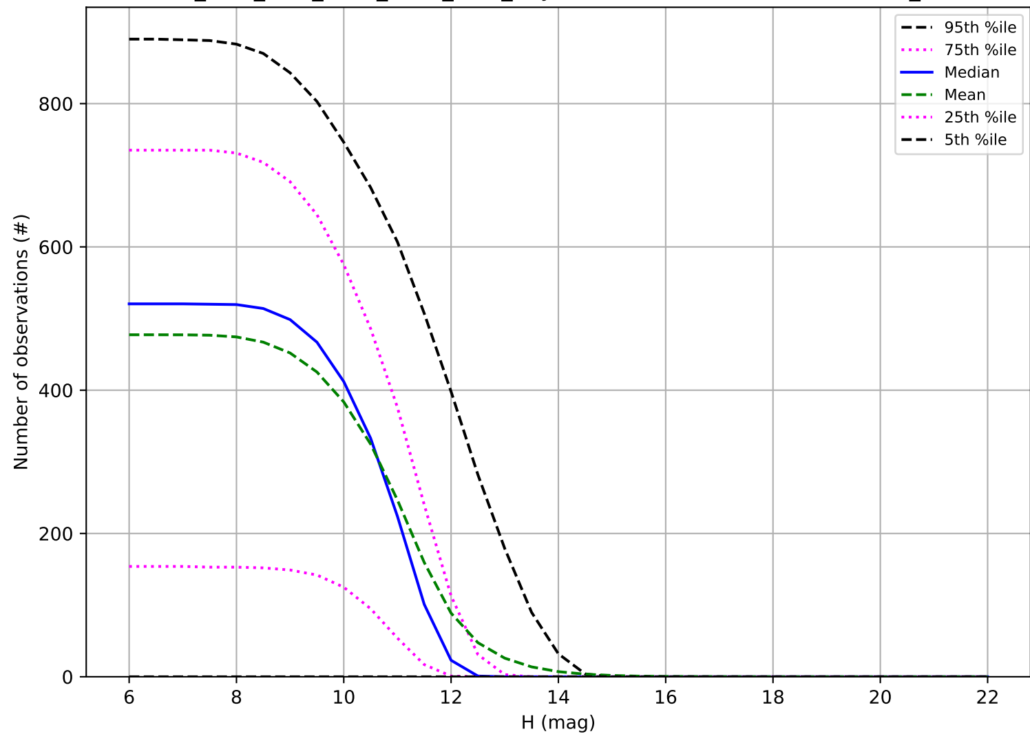
ddf_acor_sf15_lsf40_lsr10_v3.4_10yrs: Number of observations OCC_r20
