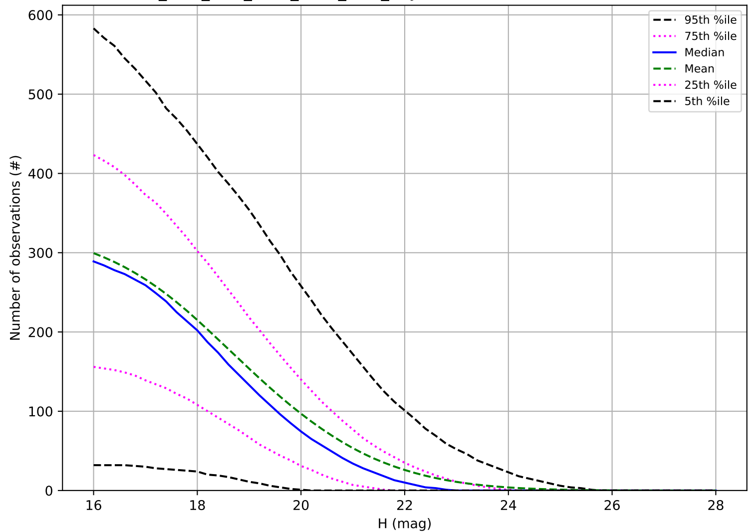
ddf_acor_sf15_lsf40_lsr10_v3.4_10yrs: Number of observations NEO
