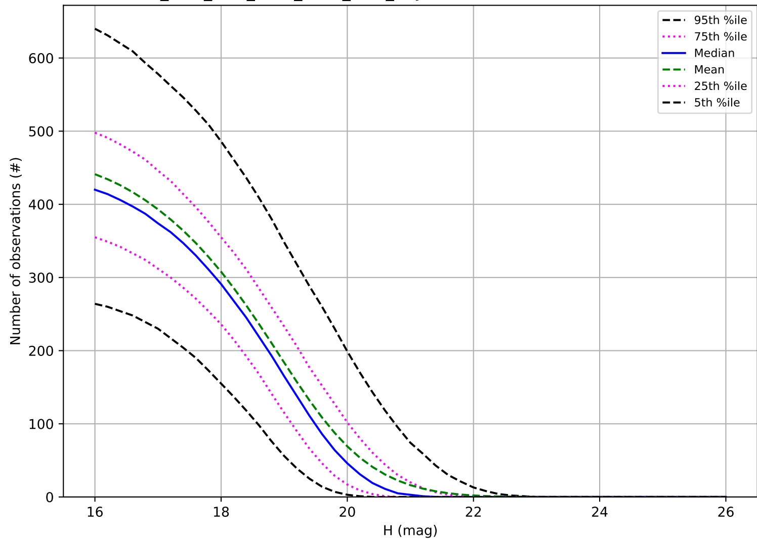
ddf_acor_sf15_lsf40_lsr10_v3.4_10yrs: Number of observations MBA
