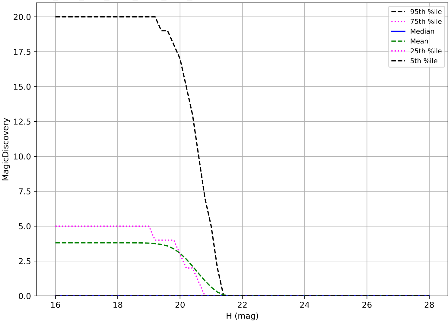
ddf_acor_sf15_lsf40_lsr10_v3.4_10yrs: Vatira 6 detections in 60 nights detection loss
