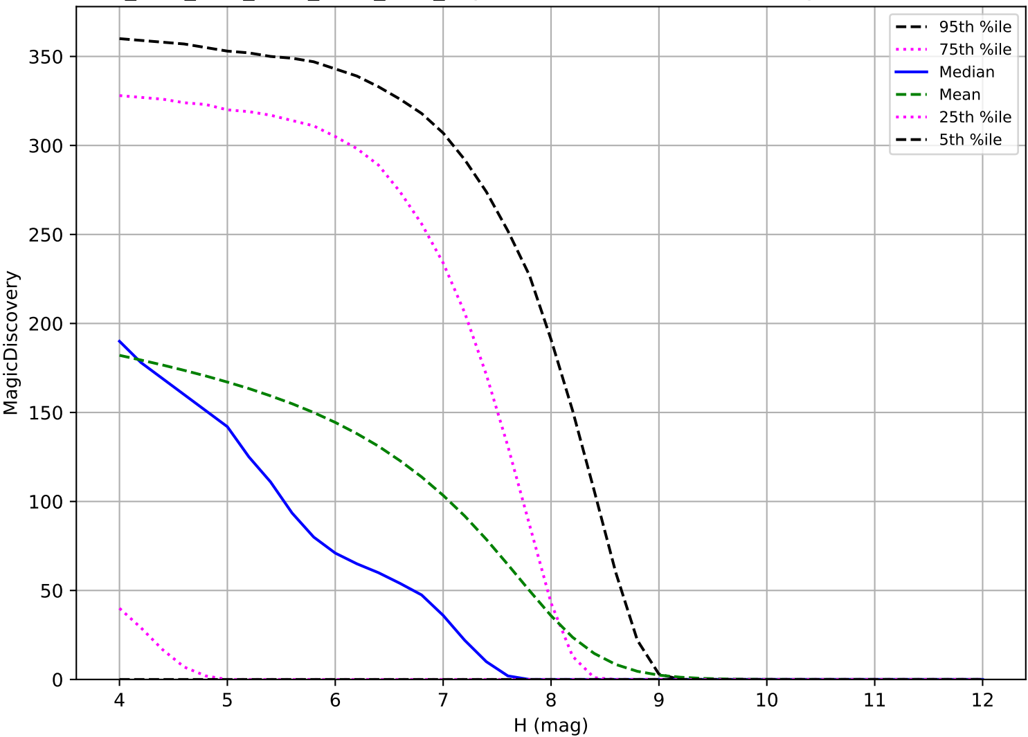
ddf_acor_sf15_lsf40_lsr10_v3.4_10yrs: TNO 6 detections in 60 nights detection loss
