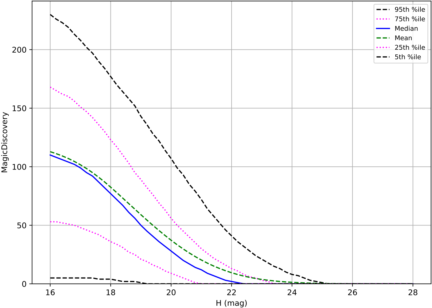
ddf_acor_sf15_lsf40_lsr10_v3.4_10yrs: NEO 6 detections in 60 nights detection loss
