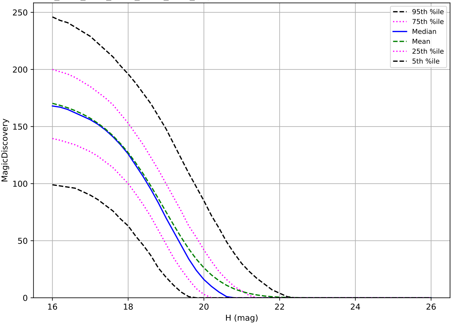
ddf_acor_sf15_lsf40_lsr10_v3.4_10yrs: MBA 6 detections in 60 nights detection loss
