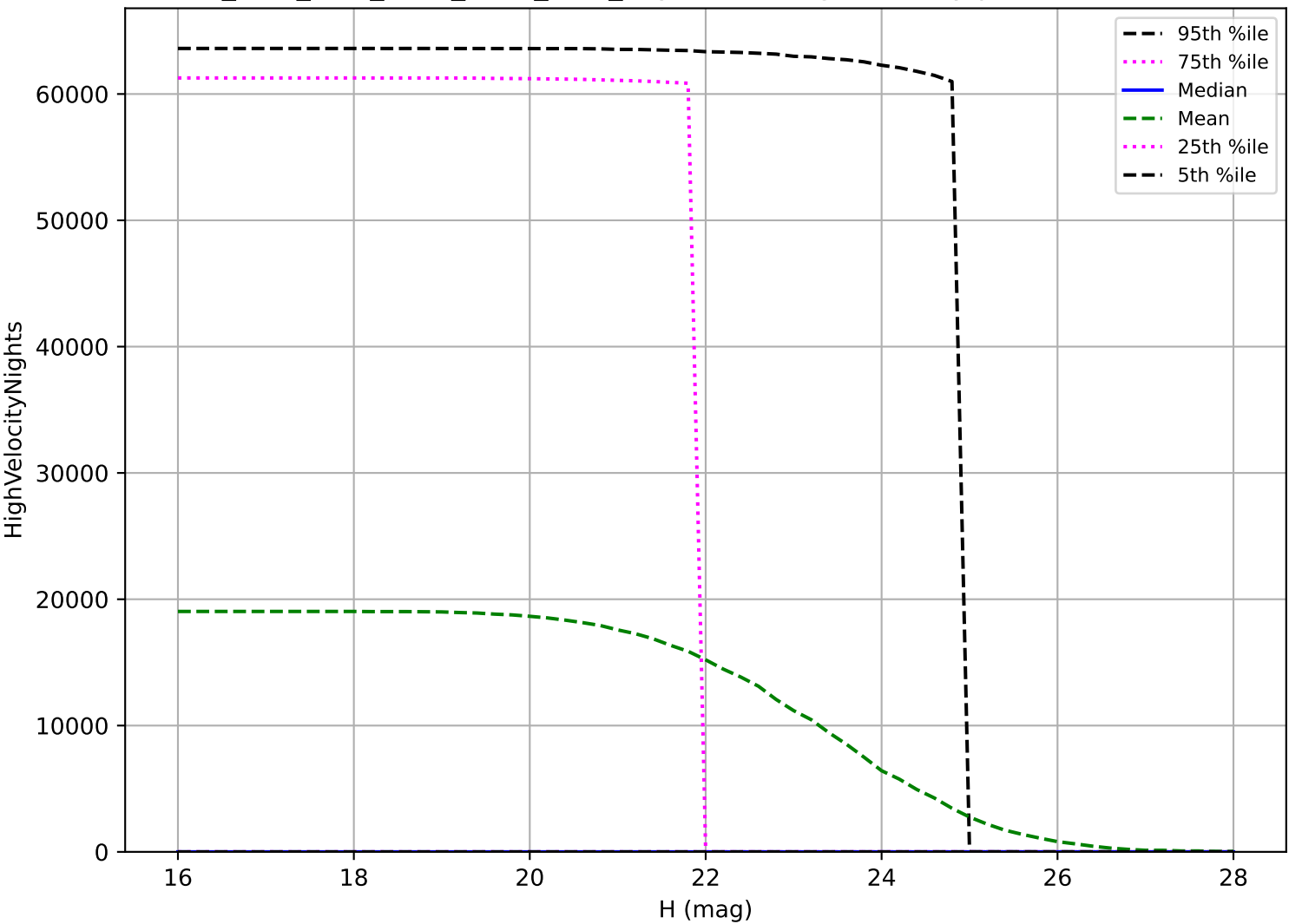
ddf_acor_sf15_lsf40_lsr10_v3.4_10yrs: NEO High velocity pair detection loss
