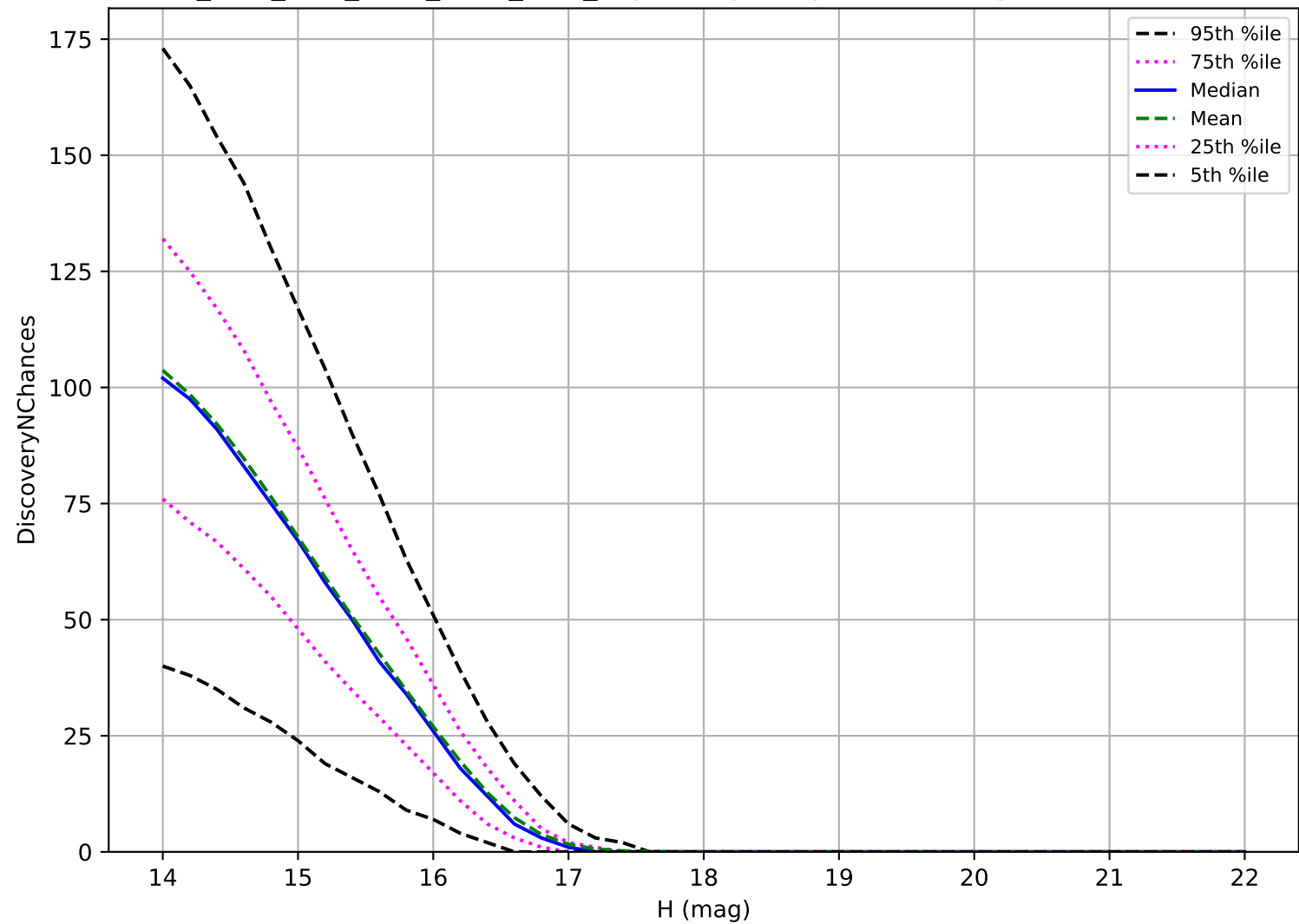
ddf_acor_sf15_lsf40_lsr10_v3.4_10yrs: Trojan 3 pairs in 15 nights detection loss
