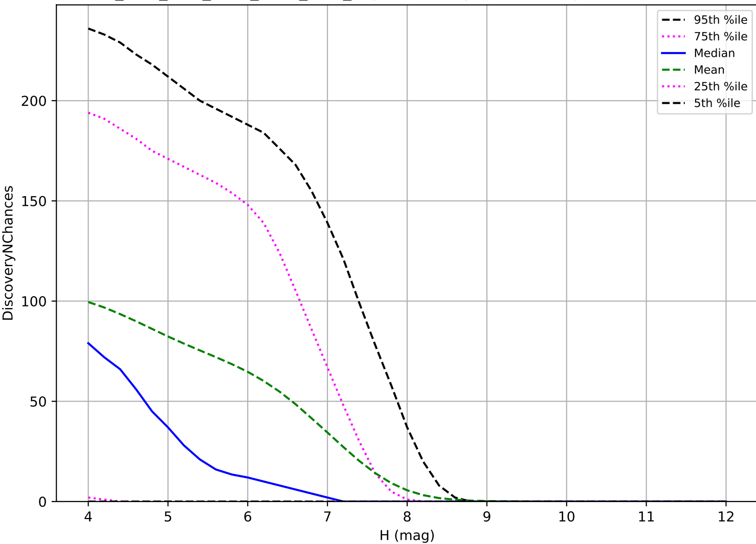
ddf_acor_sf15_lsf40_lsr10_v3.4_10yrs: TNO 3 pairs in 15 nights detection loss
