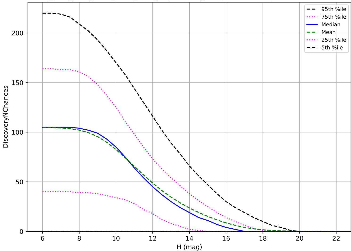
ddf_acor_sf15_lsf40_lsr10_v3.4_10yrs: OCC_r5 3 pairs in 15 nights detection loss
