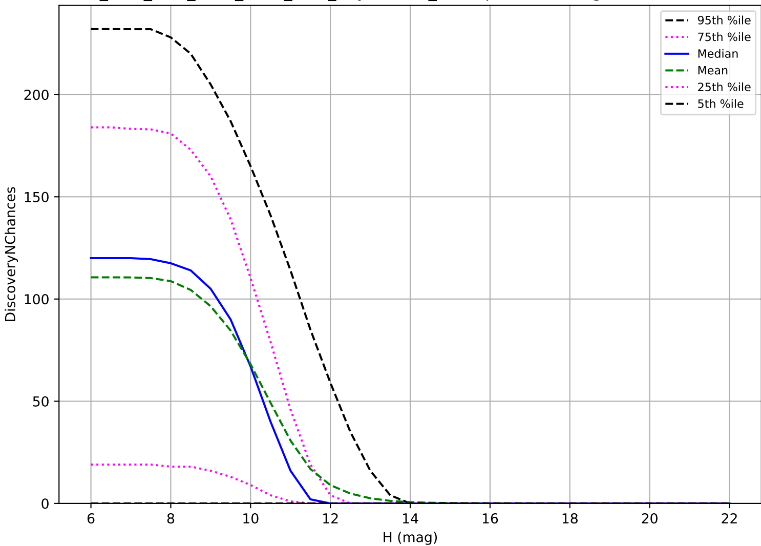
ddf_acor_sf15_lsf40_lsr10_v3.4_10yrs: OCC_r20 3 pairs in 15 nights detection loss
