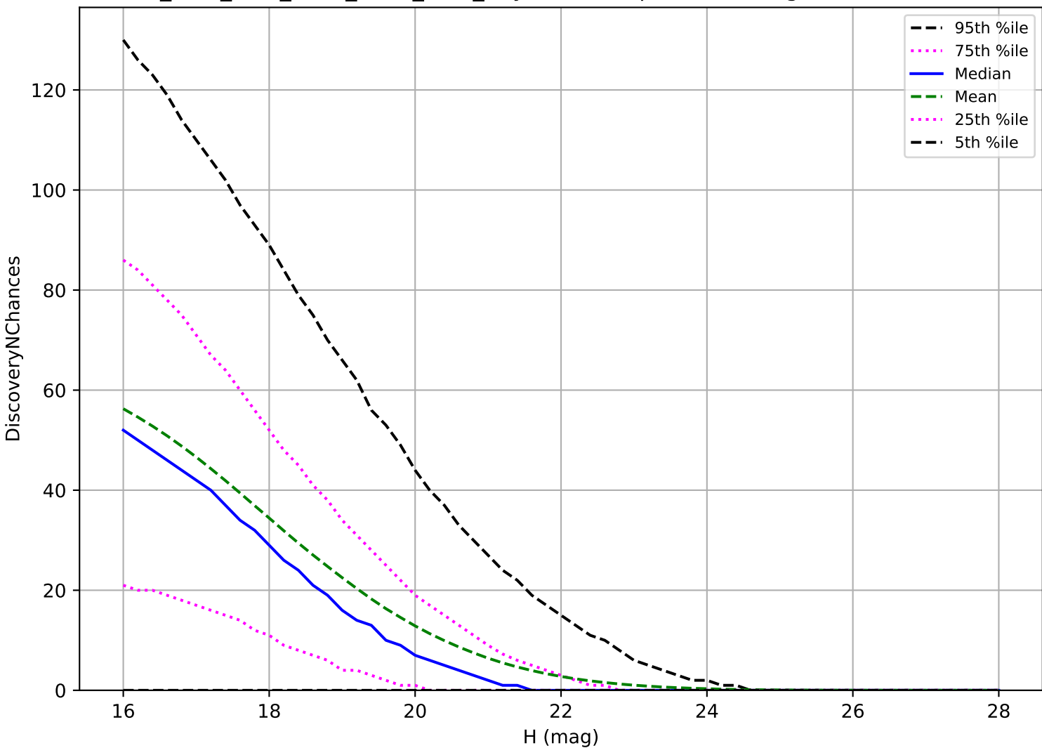
ddf_acor_sf15_lsf40_lsr10_v3.4_10yrs: NEO 3 pairs in 15 nights detection loss
