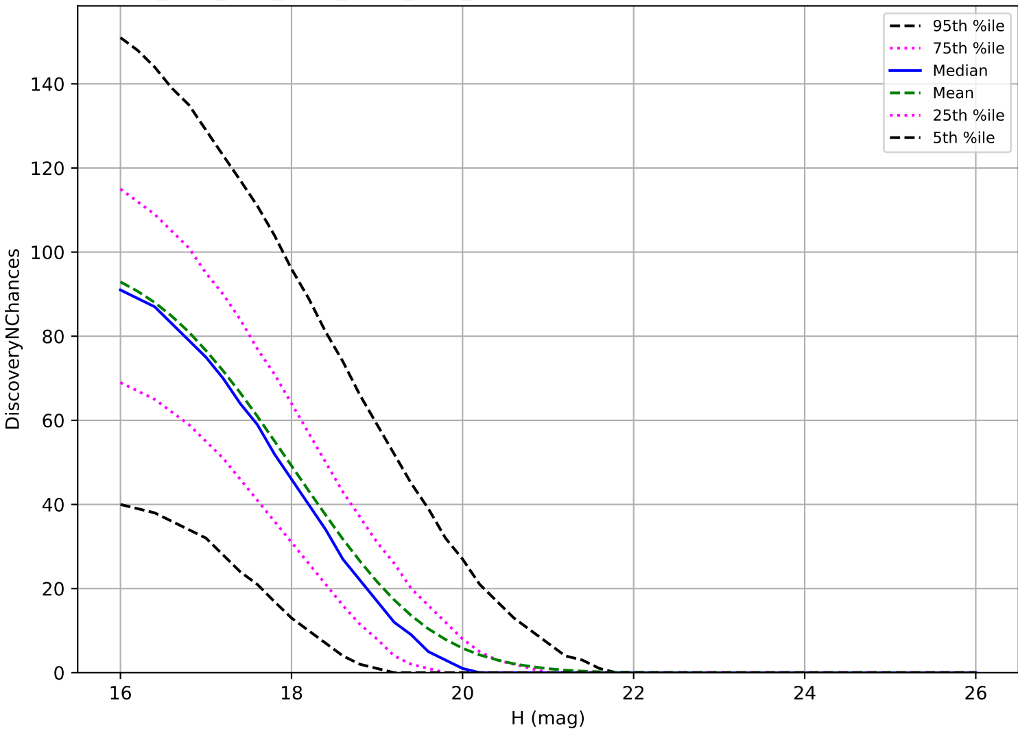
ddf_acor_sf15_lsf40_lsr10_v3.4_10yrs: MBA 3 pairs in 15 nights detection loss
