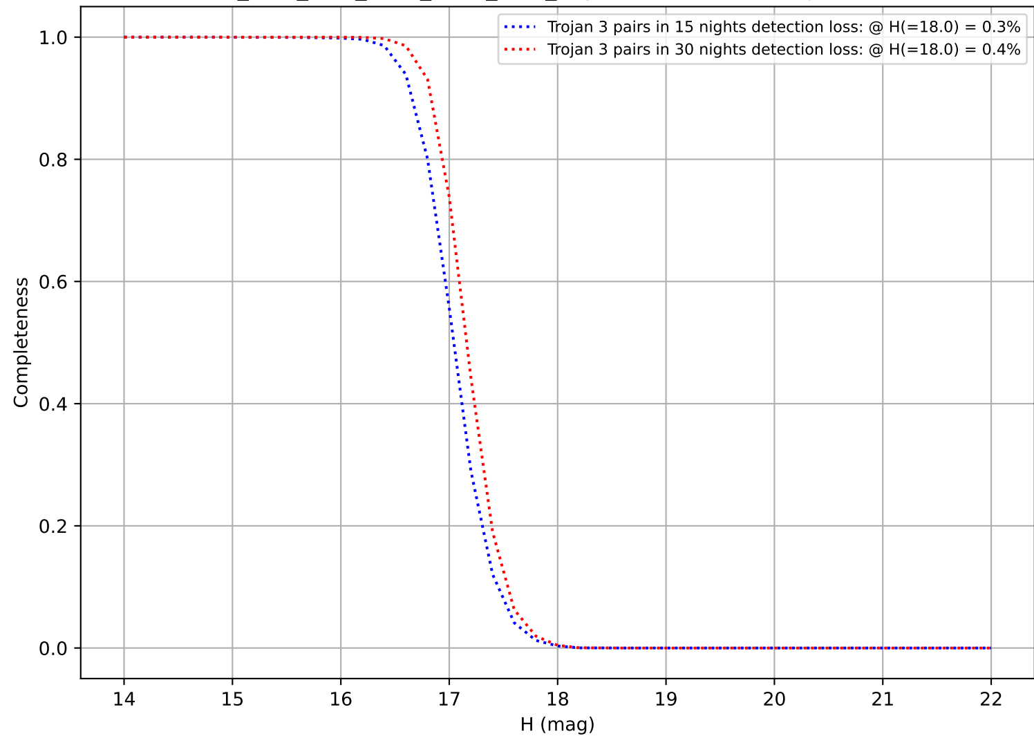
ddf_acor_sf15_lsf40_lsr10_v3.4_10yrs: DifferentialCompleteness
