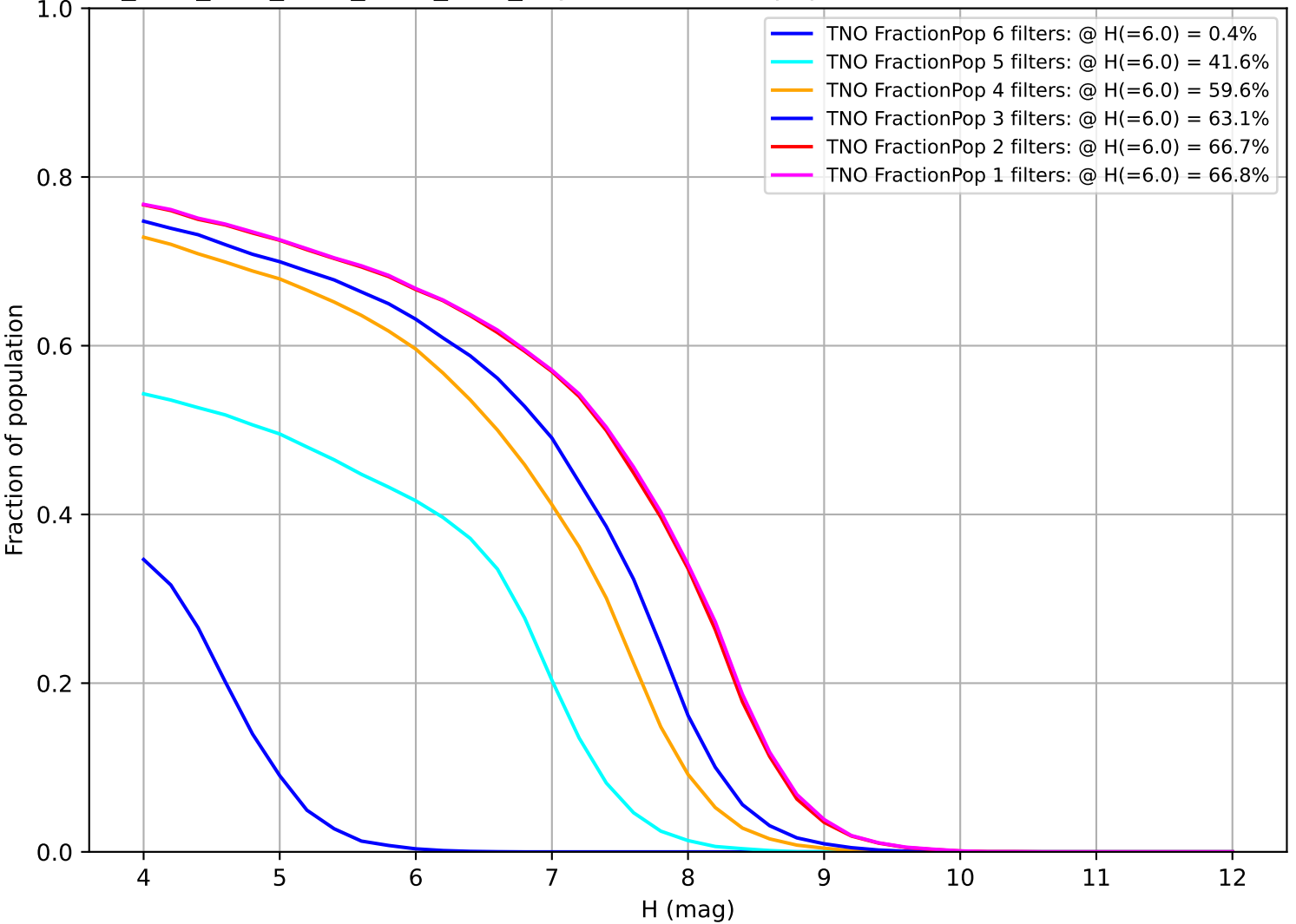
ddf_acor_sf15_lsf40_lsr10_v3.4_10yrs: Fraction of population with colors in X filters TNO
