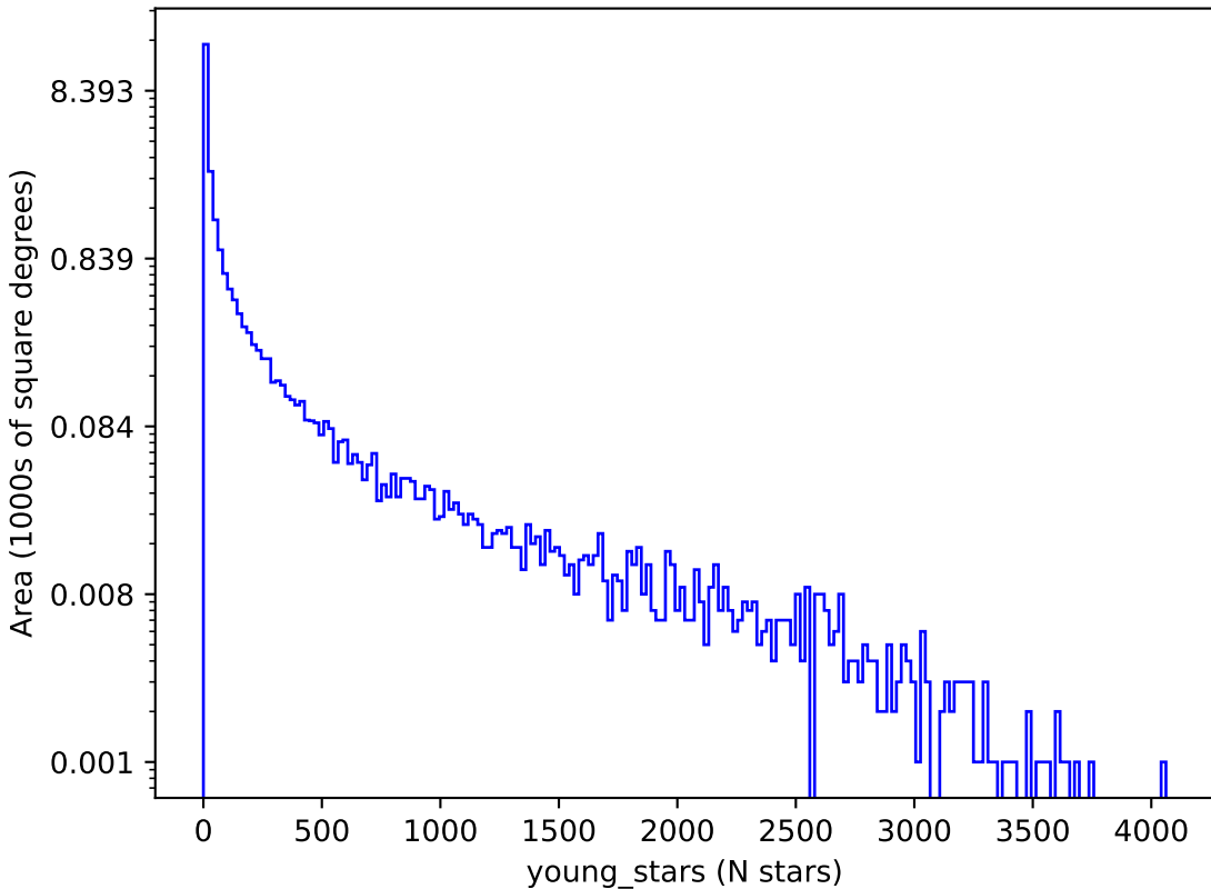
ddf_acor_sf15_lsf40_lsr10_v3.4_10yrs : young_stars
