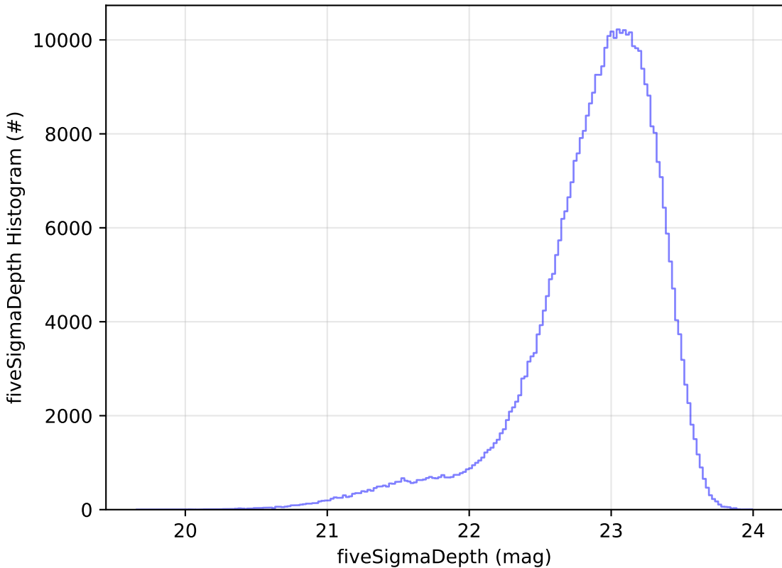
ddf_acor_sf15_lsf40_lsr10_v3.4_10yrs z: fiveSigmaDepth Histogram
