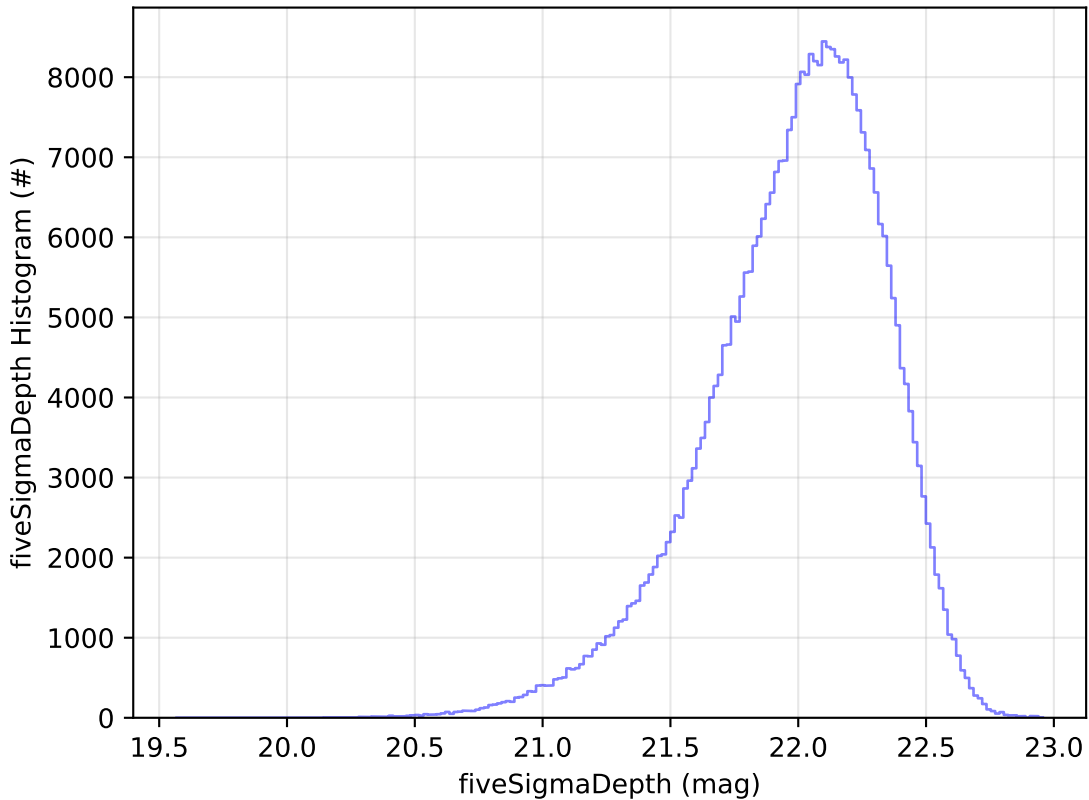
ddf_acor_sf15_lsf40_lsr10_v3.4_10yrs y: fiveSigmaDepth Histogram
