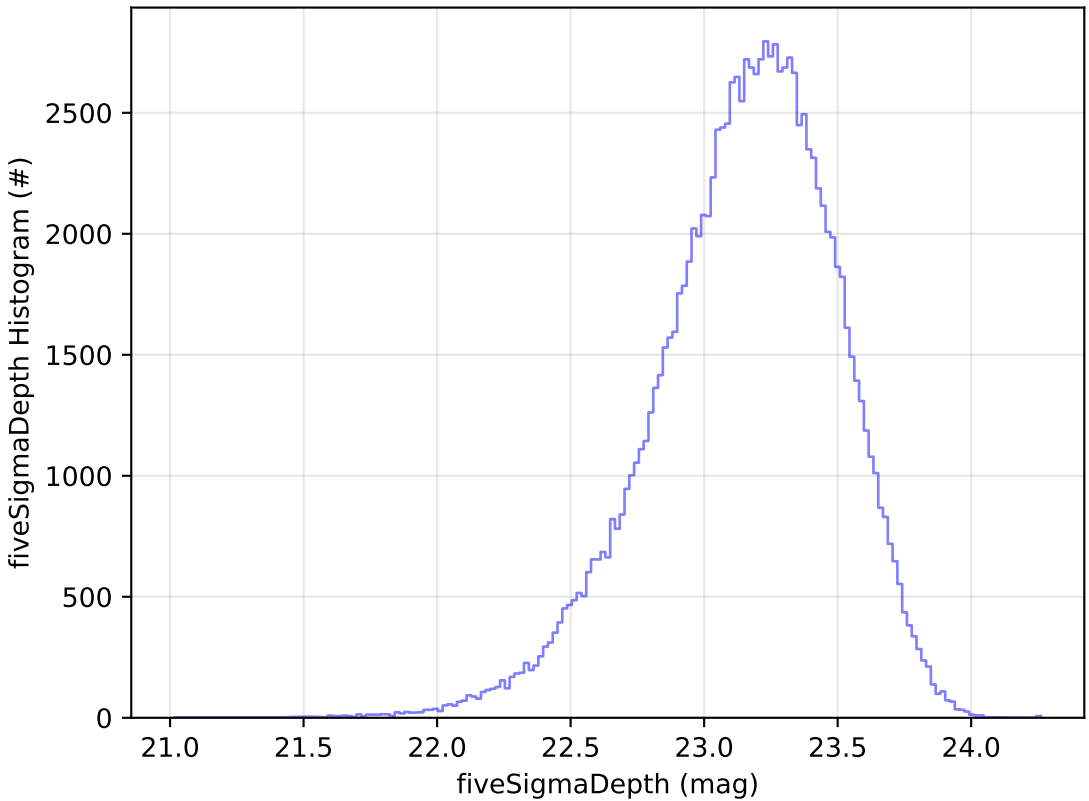
ddf_acor_sf15_lsf40_lsr10_v3.4_10yrs u: fiveSigmaDepth Histogram
