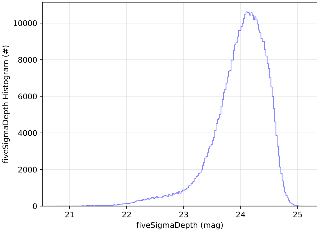
ddf_acor_sf15_lsf40_lsr10_v3.4_10yrs r: fiveSigmaDepth Histogram
