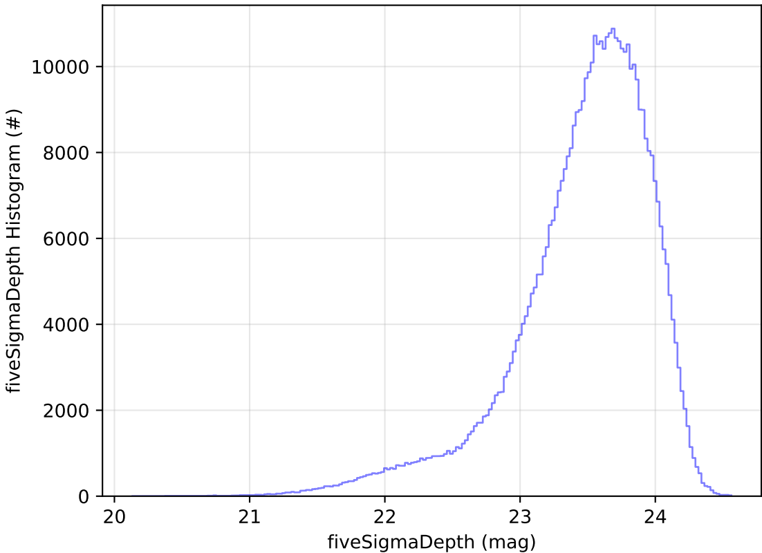
ddf_acor_sf15_lsf40_lsr10_v3.4_10yrs i: fiveSigmaDepth Histogram
