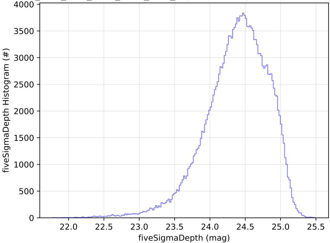
ddf_acor_sf15_lsf40_lsr10_v3.4_10yrs g: fiveSigmaDepth Histogram
