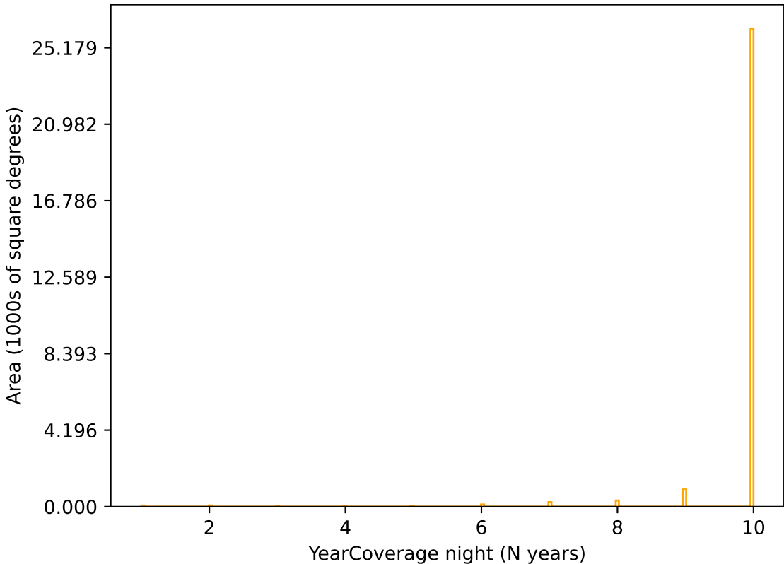
ddf_acor_sf15_lsf40_lsr10_v3.4_10yrs r band: YearCoverage night
