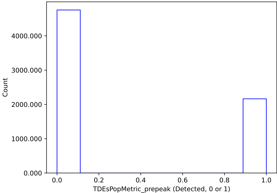
ddf_acor_sf15_lsf40_lsr10_v3.4_10yrs : TDEsPopMetric_prepeak
