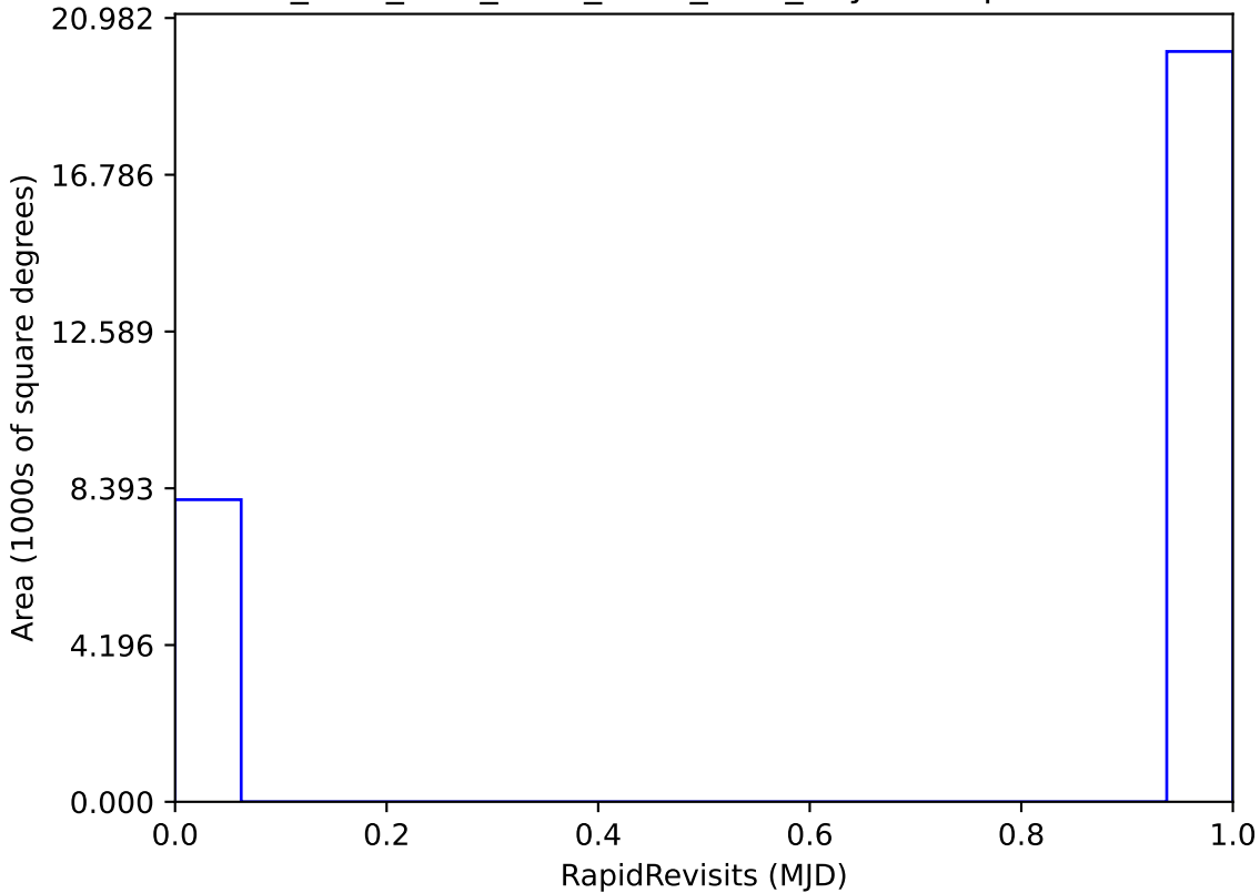
ddf_acor_sf15_lsf40_lsr10_v3.4_10yrs : RapidRevisits
