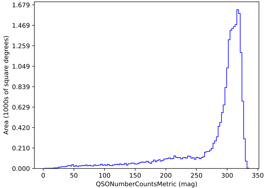
ddf_acor_sf15_lsf40_lsr10_v3.4_10yrs u band and non-DD: QSONumberCountsMetric
