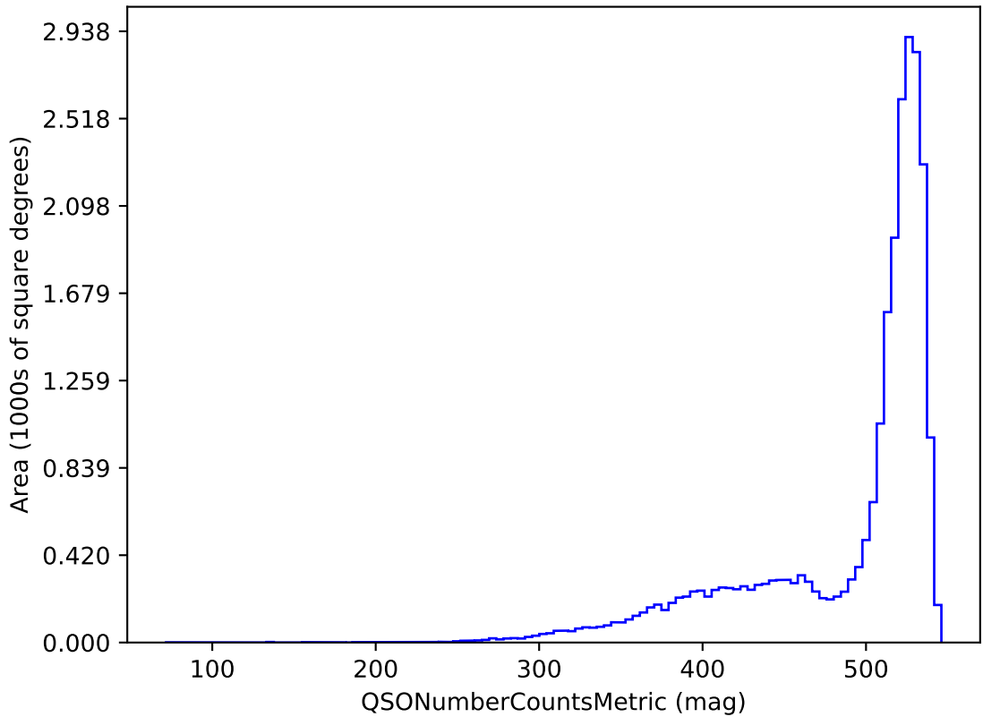
ddf_acor_sf15_lsf40_lsr10_v3.4_10yrs r band and non-DD: QSONumberCountsMetric
