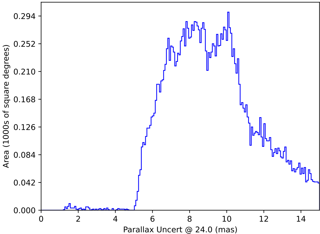
ddf_acor_sf15_lsf40_lsr10_v3.4_10yrs : Parallax Uncert @ 24.0
