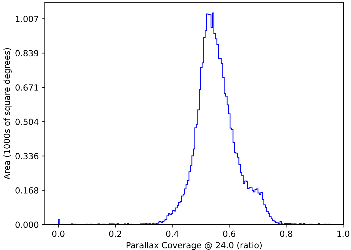
ddf_acor_sf15_lsf40_lsr10_v3.4_10yrs : Parallax Coverage @ 24.0
