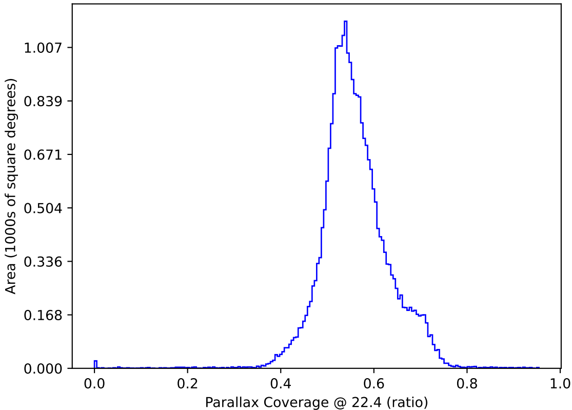
ddf_acor_sf15_lsf40_lsr10_v3.4_10yrs : Parallax Coverage @ 22.4
