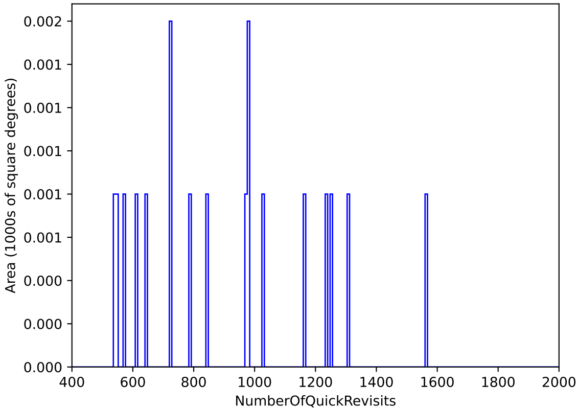
ddf_acor_sf15_lsf40_lsr10_v3.4_10yrs : NumberOfQuickRevisits
