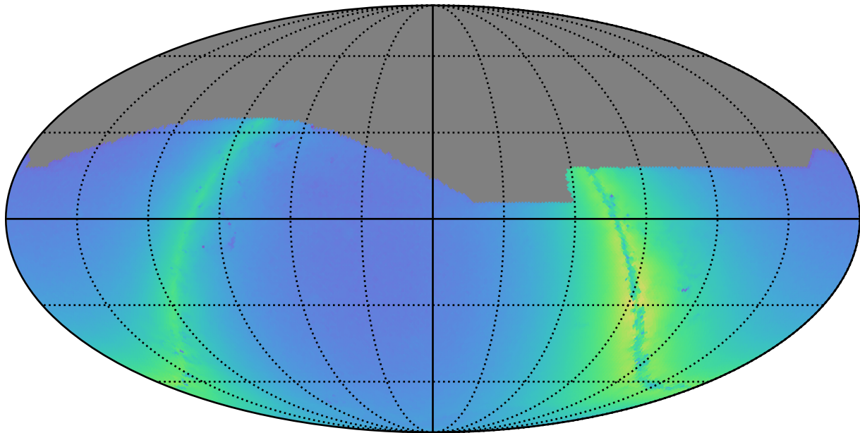
ddf_acor_sf15_lsf40_lsr10_v3.4_10yrs r: Nstars_no_crowding
