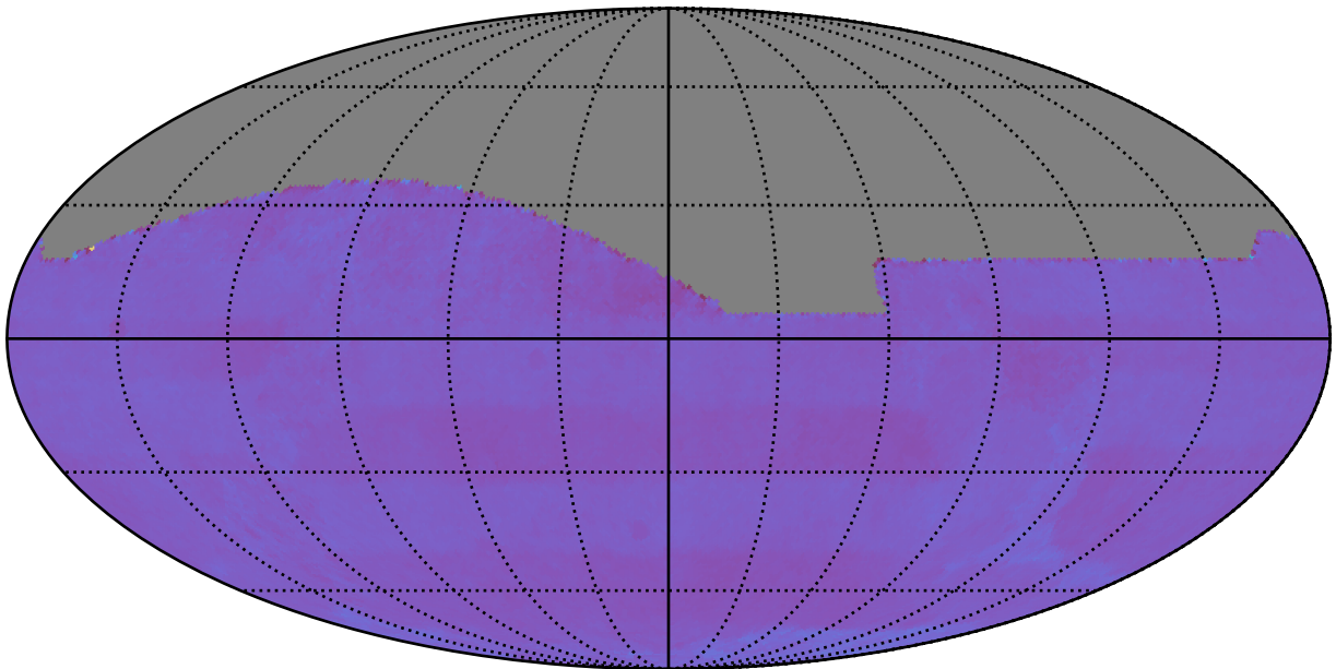
ddf_acor_sf15_lsf40_lsr10_v3.4_10yrs : Normalized Proper Motion Uncert @ 24.0
