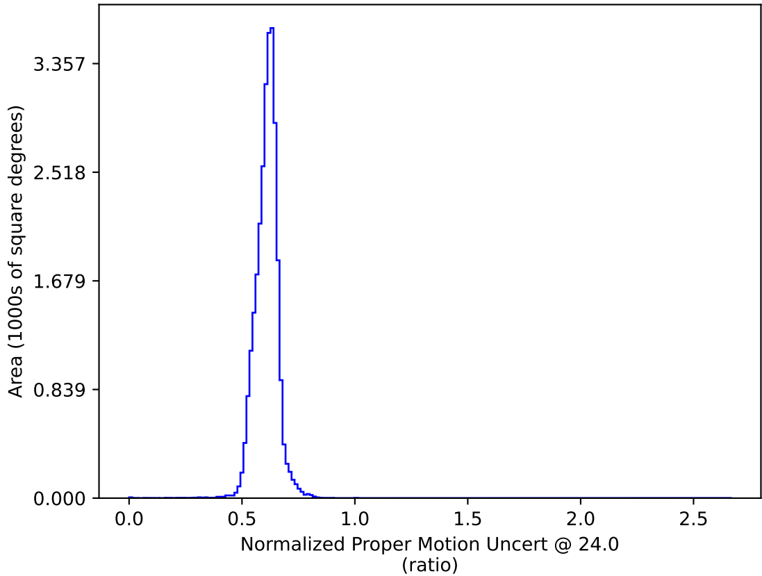
ddf_acor_sf15_lsf40_lsr10_v3.4_10yrs : Normalized Proper Motion Uncert @ 24.0
