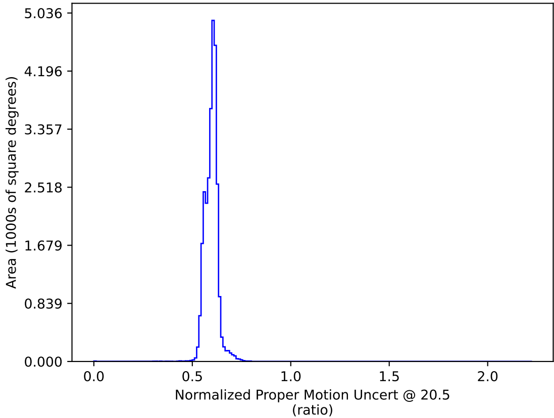
ddf_acor_sf15_lsf40_lsr10_v3.4_10yrs : Normalized Proper Motion Uncert @ 20.5
