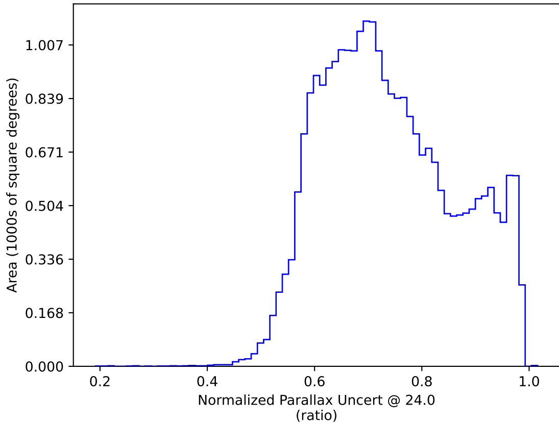
ddf_acor_sf15_lsf40_lsr10_v3.4_10yrs : Normalized Parallax Uncert @ 24.0
