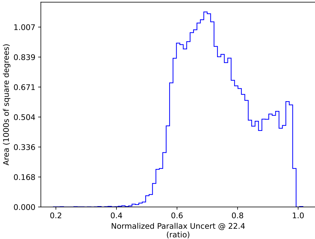
ddf_acor_sf15_lsf40_lsr10_v3.4_10yrs : Normalized Parallax Uncert @ 22.4
