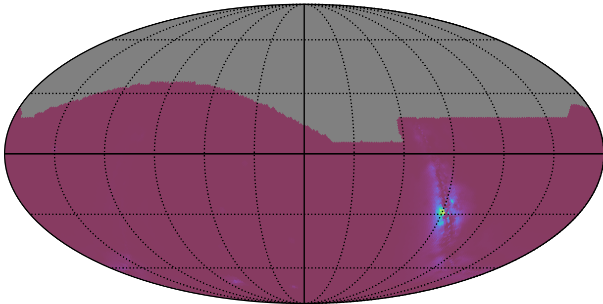
ddf_acor_sf15_lsf40_lsr10_v3.4_10yrs : NlcPoints
