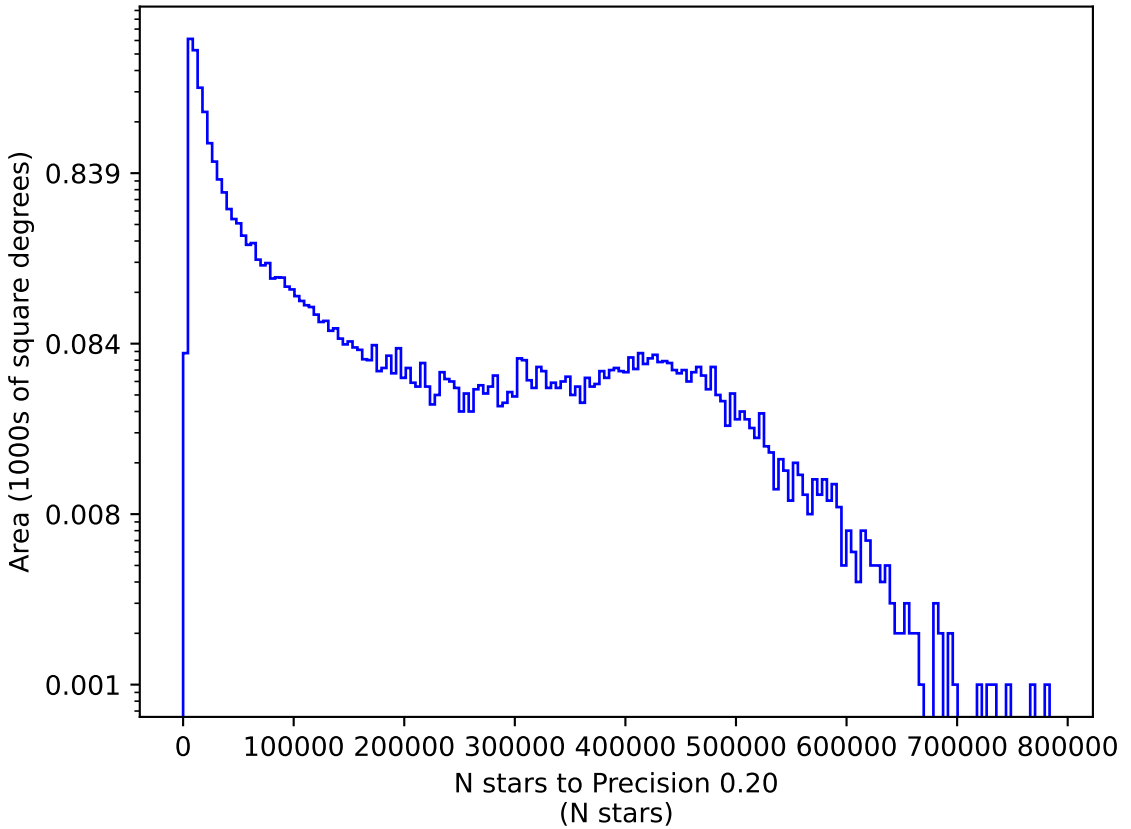
ddf_acor_sf15_lsf40_lsr10_v3.4_10yrs r: N stars to Precision 0.20
