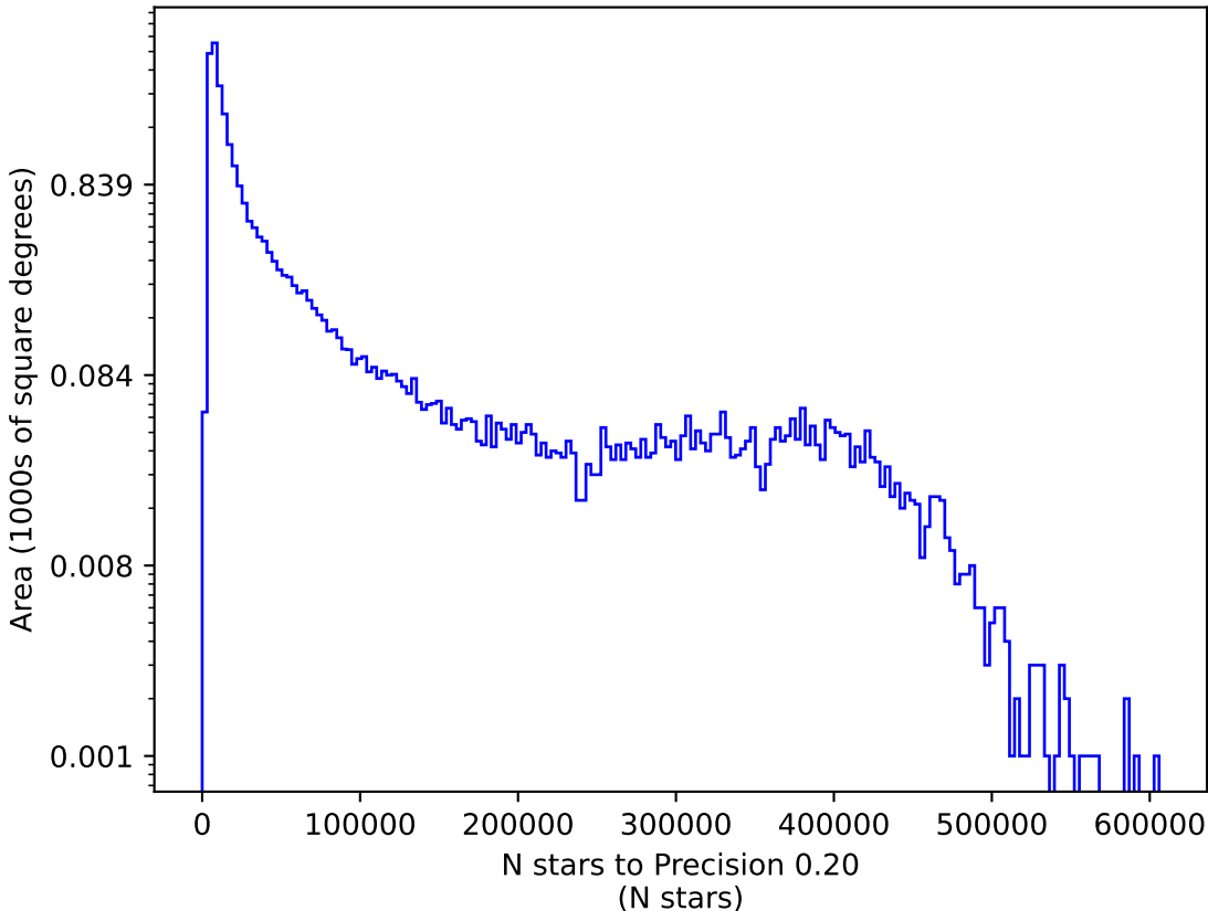
ddf_acor_sf15_lsf40_lsr10_v3.4_10yrs g: N stars to Precision 0.20
